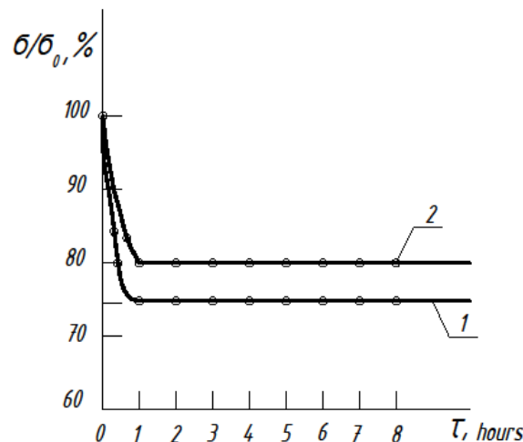
Figure 1. Stress change in specimens at the initial stage 1 – stress amplitude of 10 kg/mm 2 ; 2 – stress amplitude of 5 kg/mm 2 .
