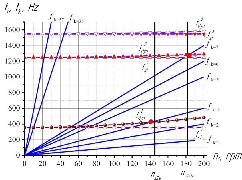
Figure 3. Campbell diagram for LPT stage 1 rotor blade of D-36 engine [Error! Reference source not found.].
