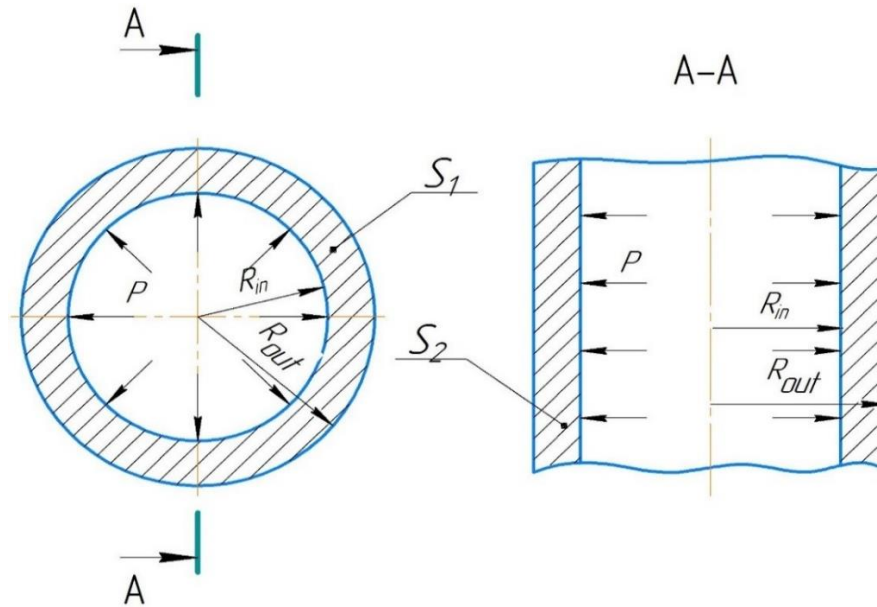
Figure 4. Geometric parameters.
