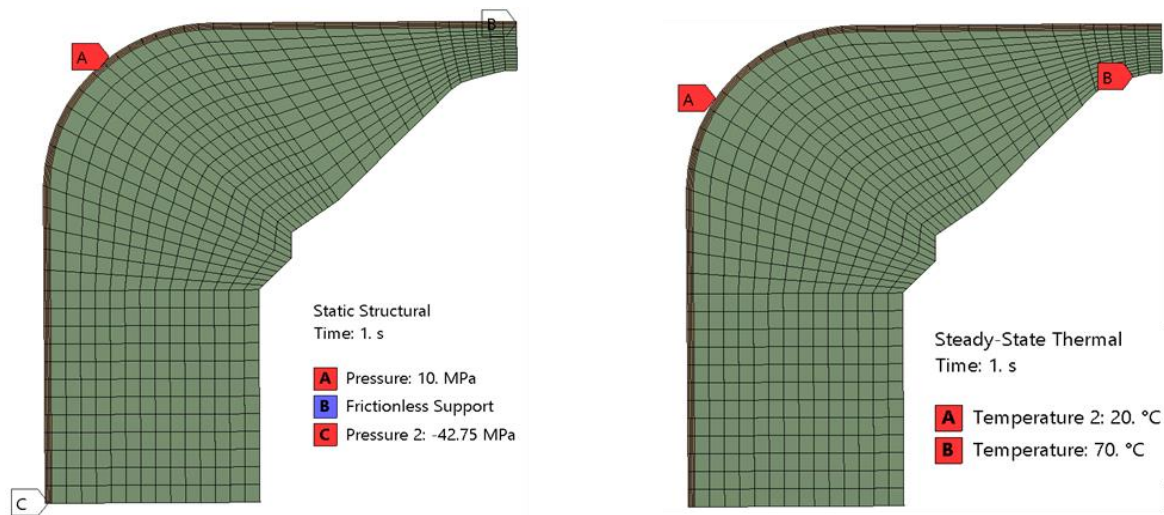
Figure 2. Finite element model and applied boundary conditions for the stress transformation approach.
