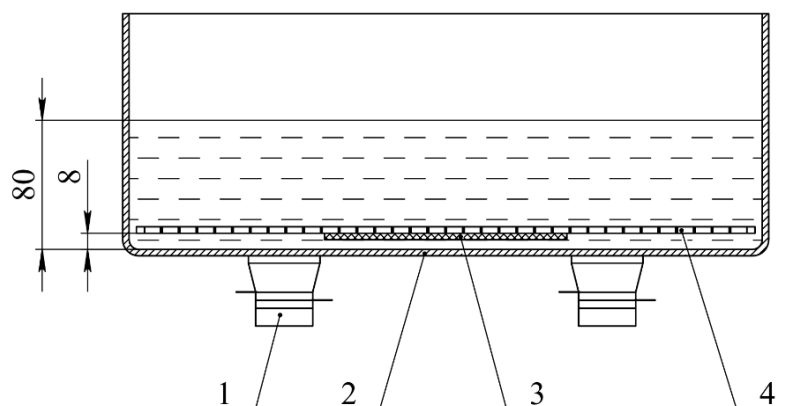
Legend: 1 – ultrasonic emitter; 2 – liquid container; 3 – experimental sample; 4 – retaining grid.
