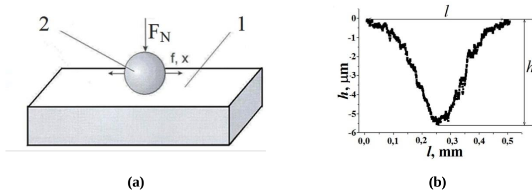
Figure 1. Schematic representation of the friction tests: (a) oscillatory sliding of a counterbody made of a steel or ceramic ball on the surface of hardened VT6 alloy and (b) typical cross-sectional geometry of a wear track of depth h and width l . 1 – polished specimen surface; 2 – counterbody (ball rigidly fixed to the loading beam); F_N – applied normal force.
