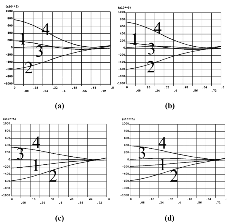
Figure 5. Graphs of stress magnitude along the strip layer above and below the contact line: (a) For condition of slippage with possible lag, above the contact line without friction; (b) For condition of slippage with possible lag above the contact line with friction; (c) For condition of slippage with possible lag below the contact line without friction; (d) For condition of slippage with possible lag below the contact line with friction; \sigma_x – line 1, \sigma_y – line 2, \sigma_{xy} – line 3, \sigma_i – line 4.
