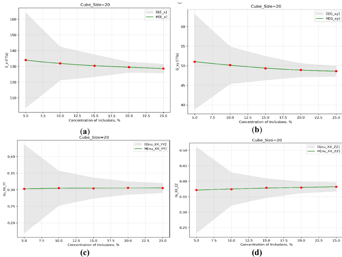
Figure 3. Dependence of elastic properties: a) Young's modulus E_x ; b) shear modulus G_{xy} ; c) Poisson's ratios \nu_{xxyy} ; d) \nu_{xxzz} on the concentration of inclusions at a fixed size of 20 voxels.
