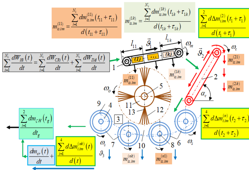
Figure 5. Model scheme for calculating the phased separation of impurities from root crops by working bodies of the CTM: 1 – inclined conveyor; 2 – cleaning slide; 3 – combined working body; 4 – cleaning screws; 5 – cleaning shaft; 6, 7 – respectively, right and left system; 8 – screw shaft; 9 – lower branch of the ellipse; 10 – working channel chute; 11 – drum; 12 – elastic cleaning elements; 13 – pile bundles.
