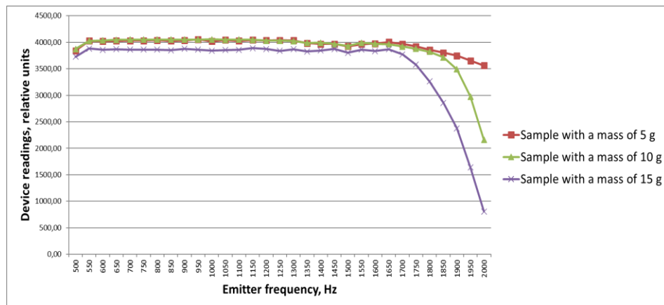
Figure 8. Dependence of the device readings on the emitter frequency for samples of different masses with the highest linear density.
