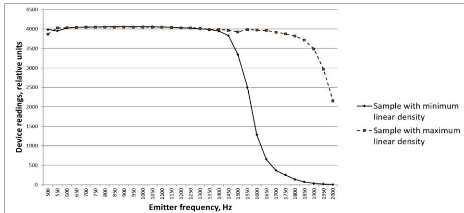
Figure 9. Dependence of device readings on emitter frequency for samples with different linear densities.
