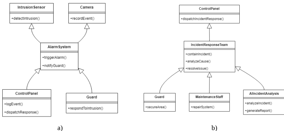
Figure 3. a – Intrusion Detection and Response Pattern, b – Incident Response Pattern
