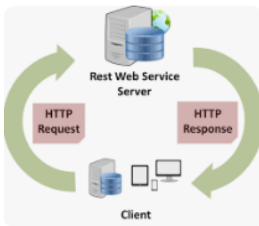
Рис. 2.2. Restful services
