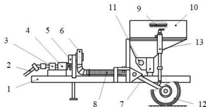
Figure 1. Schematic diagram of a pneumatic rod machine for dispersing solid mineral fertilizers:
