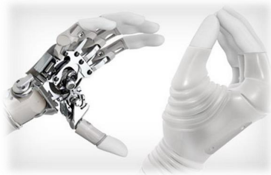
Figure 2. Appearance of the «Michelangelo hand» prosthesis [6, 7].
