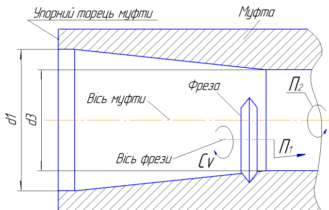
Figure 1. Model milling of internal screw-thread in general
