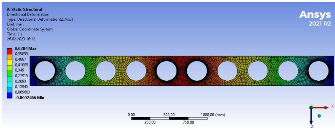
Figure 17. Estimated deflection of a cellular beam, mm (ANSYS, beam model with finite elements mesh refinement near the edge of the selected holes)
