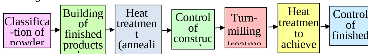
Figure 3 - Prospective scheme for the manufacture of products using the additive technologies
