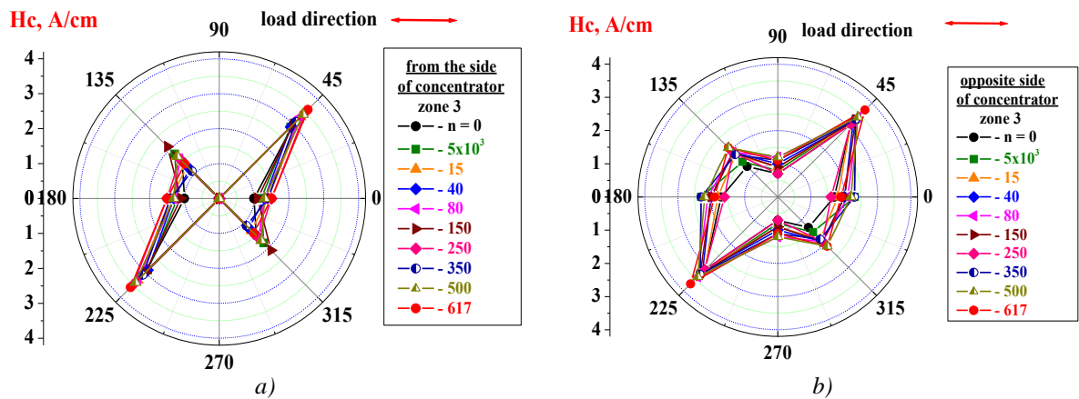
Figure 23. The diagrams of the coercive force values distribution along two sides of the continuous parts (without opening) between the working part edge and the opening (a), and on the opposite sample side (b)
