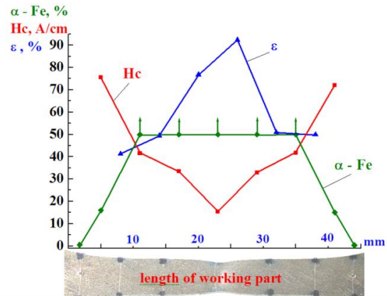
Figure 12. Distribution of the ferromagnetic phase ( \alpha -Fe) fraction, the coercive force H_c , and accumulated deformations \varepsilon along the sample working length after fracture under tension
