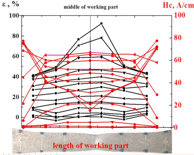
Figure 10. The distribution of deformations \varepsilon (black lines) and the coercive force H_c (red lines), measured by means of D12 sensor, along the length of the sample working part under tension
