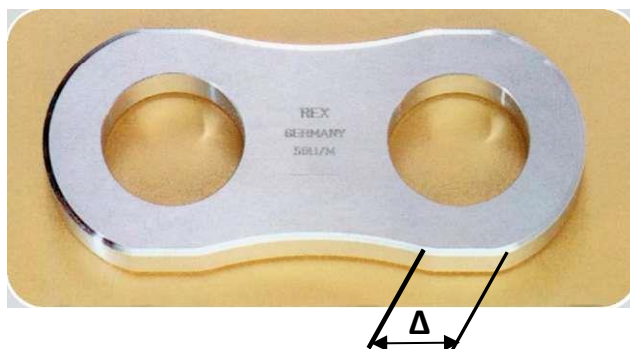
Figure 3. Plates with „flattenings“ – plate side edges containing sections with curved and flat surfaces ( \Delta ) (firm Rexnord Kette GmbH – [2])
