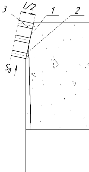
Figure 5. The profiles of grinding wheels
