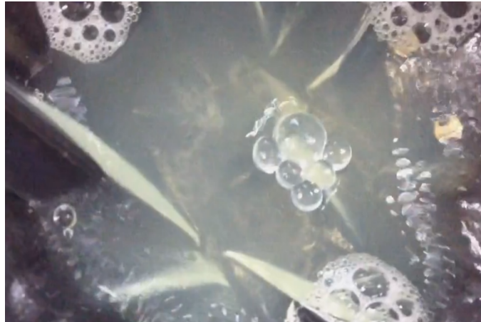
Fig. 2 The group of drops
