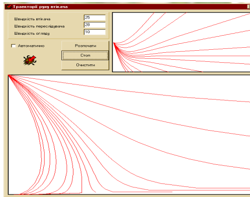
Fig.2 The interface of the program, which allows to explore the dependence of the distance and the trajectories of movement of the chaser and the fleeing person from time
