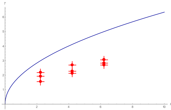
Fig. 2. Blue line – theoretical dependence between the oscillation period and ring's radius. T = 2\pi \sqrt{\frac{R}{g}}
