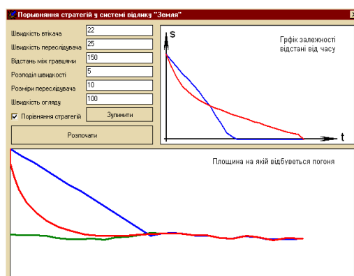
Fig.1 The interface of the program, which is modeling the persecution in reference frame Bin S and L-strategies
